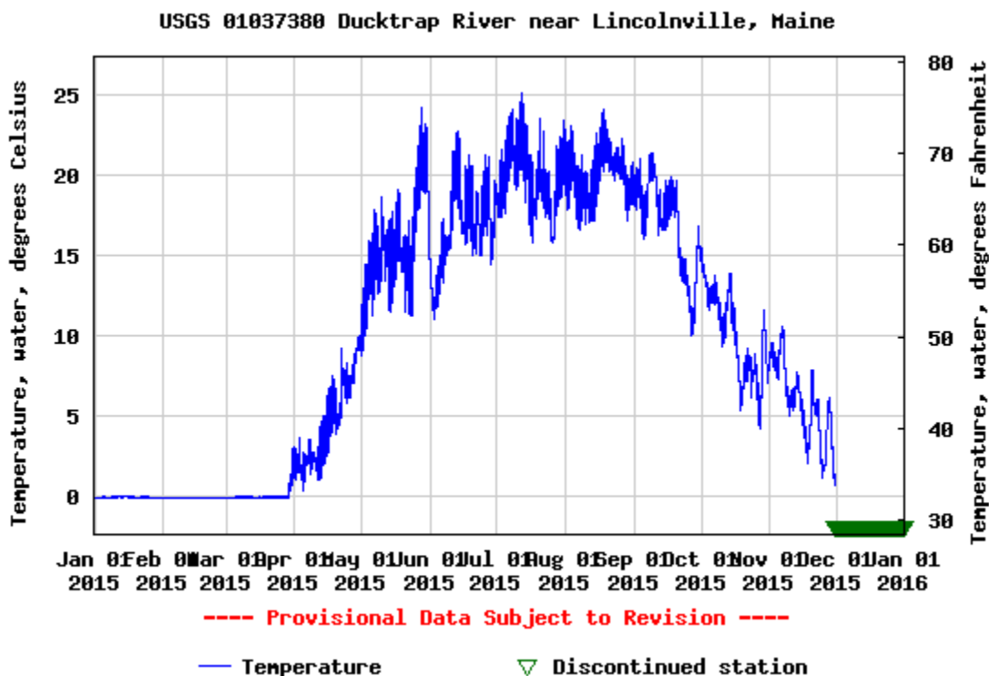
Figure 2. Daily water temperature for the Ducktrap River from the USGS gauge in Lincolnville.
