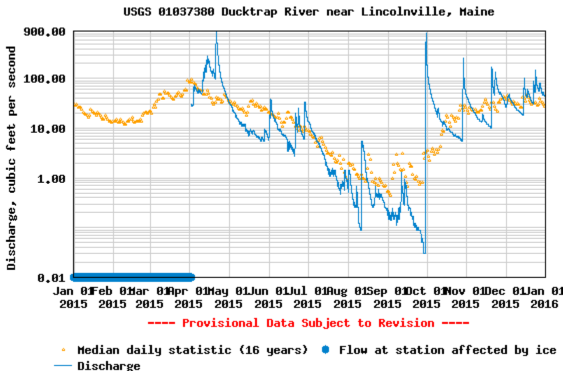
Figure 1. Ducktrap River flows for 2015 measured in Lincolnville, Maine as recorded by the USGS stream gauge. Actual measured flows are in blue, while the 16 year median is in yellow. Ice cover January-April is indicated by dark blue dots.
